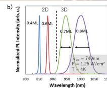
Control of 2D/3D Structures by SML growth (AFM/PL)
