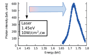
1.45eV photons (855nm) upconverted to 1.72eV (721nm)
